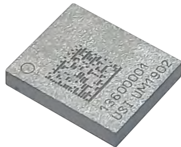
SiP模块L6.1mm W5.1mmH1.1 mm
